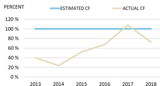
Figure 18: Comparison of estimated and actual conversion factor (CF) – mortgage loans (limit loans)
