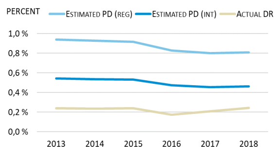
Figure 14: Comparison of unweighted estimated PD with actual DR – mortgage loans (regulatory and internal)
