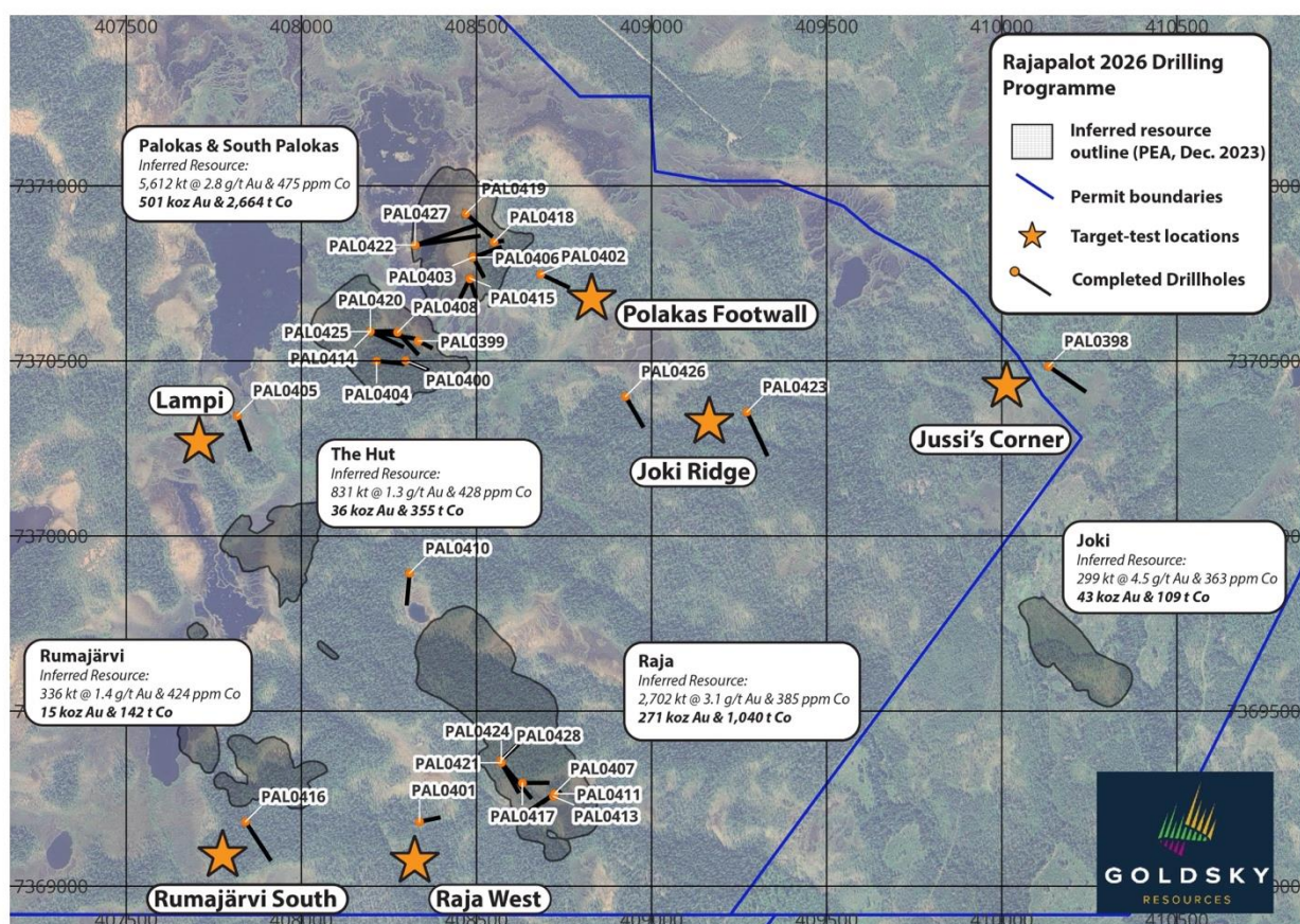
Figure 1. Drilling update from the Rajapalot project 2026 winter drilling campaign. To date, a total of 6,073 metres of drilling has been completed from 31 drillholes. A total of 4,727 metres of infill drilling has been completed from 23 drillholes, while a total of 1,346 metres of Target Test drilling from 8 drillholes.
