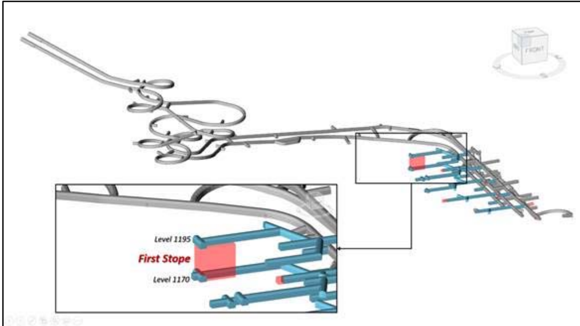
Figure 1. First transverse long hole production stope was mined between the 1195 and 1170 levels
