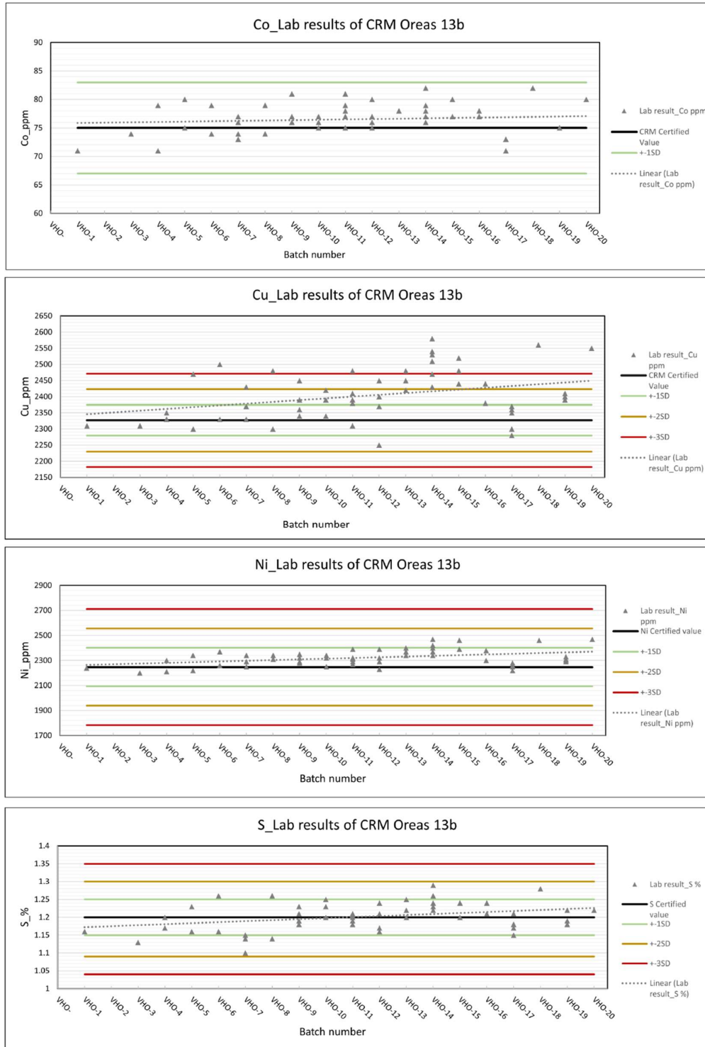
Figure 8-5 Assay results of standard Ores 13b, in chronological order.
