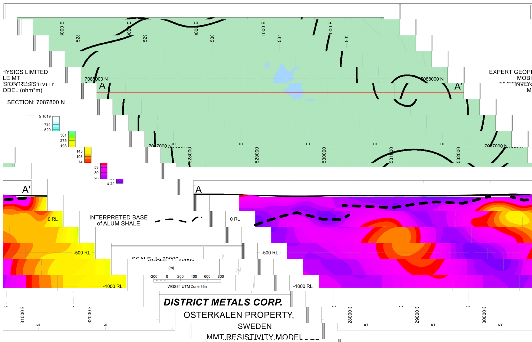
Figure 2: Cross Section through MobileMT Low Resistivity Anomaly at Österkälén Property
