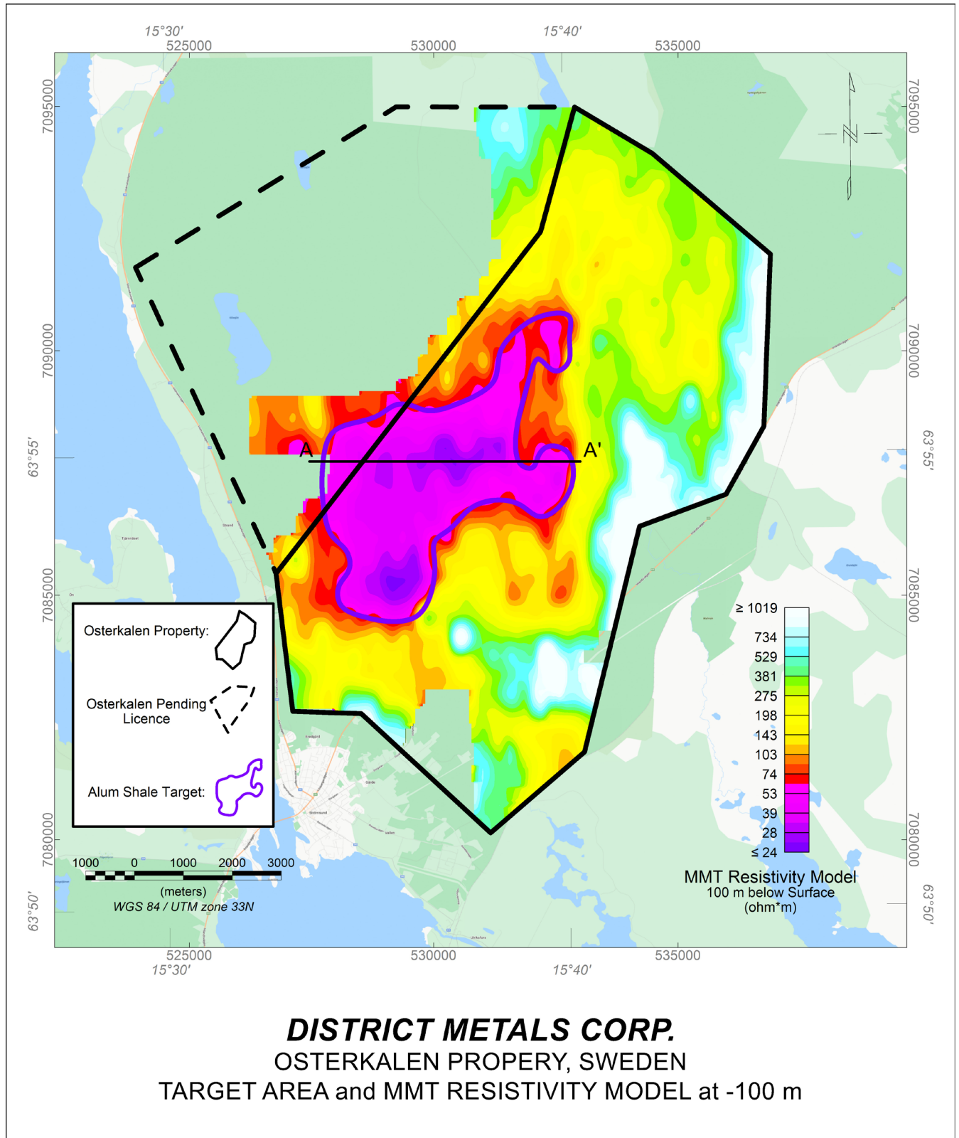
Figure 1: Österkalen Property MobileMT Survey Results in Plan View
