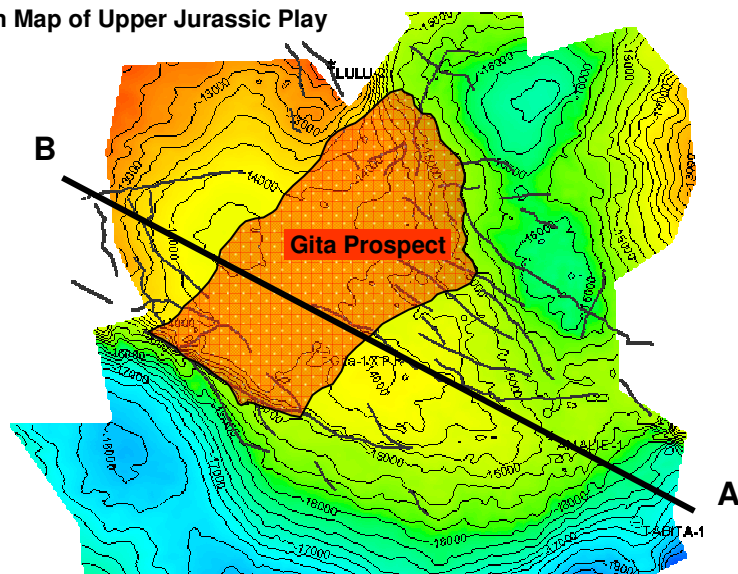
Depth Map of Upper Jurassic Play
